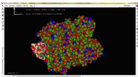
Figure 10: After docking the Receptor and the Ligand Methylanthralene
