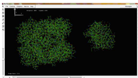
Figure 9: Receptor and the Ligand ready for docking
