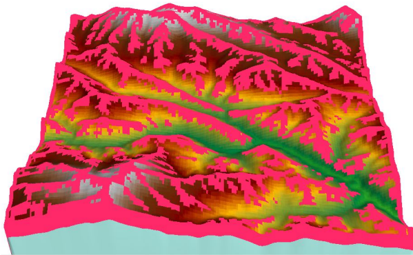
Fig.3.9 Mountain Tops, High Ridges
