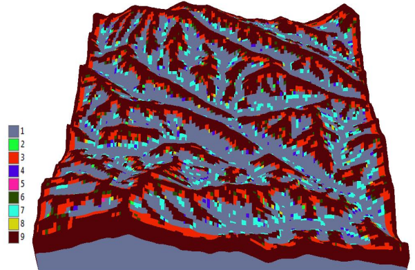
Figure 4. Landform classification map for the study area
