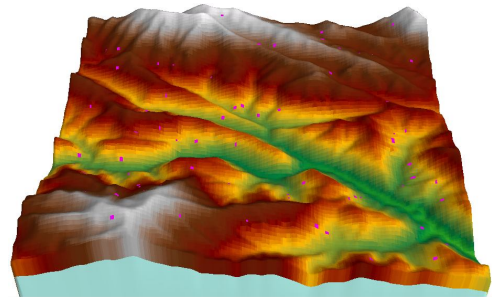
Fig.3.8 Midslope Ridges, Small Hills in Plains
