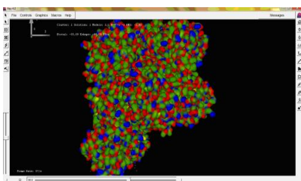
Figure 10: After docking the Receptor and the Ligand Methylanthralene
